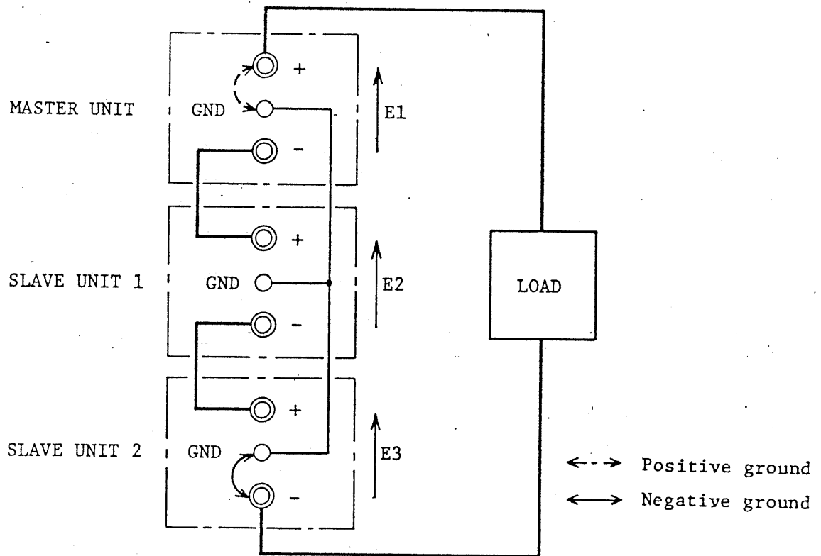
Figure 4-13. Rear output terminal connections
